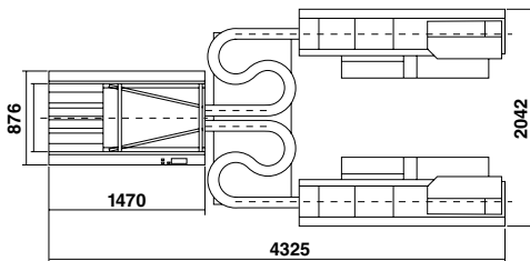
Dual Output Converger + Two Weigh-Price-Labellers
