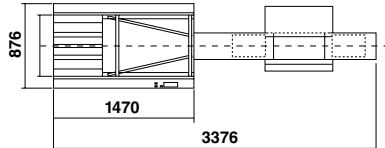
Dual Output Converger + Two Weigh-Price-Labellers
